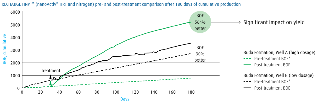
Fig. 5 Cumulative BOE production at the Buda wells before and after treatment with N 2 and nanoActiv® HRT (nanoparticles)
