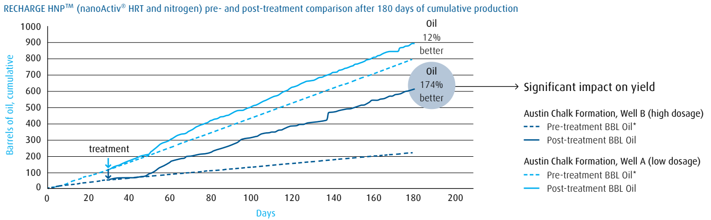
Fig. 4 Cumulative oil production for the Austin Chalk wells before and after treatment with N 2 and nanoActiv® HRT (nanoparticles)
